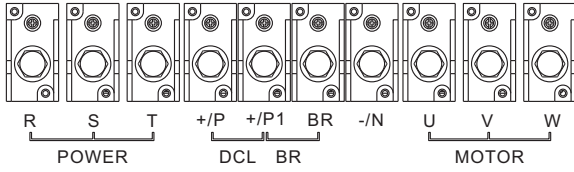
Size G(380V)(93~132kW)
