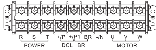
Size F(380V)(37~75kW)
