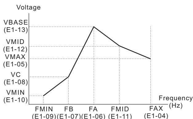
Fig. Custom V/F Pattern
