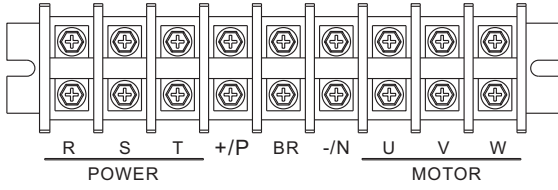
Size E(380V)(30kW)
