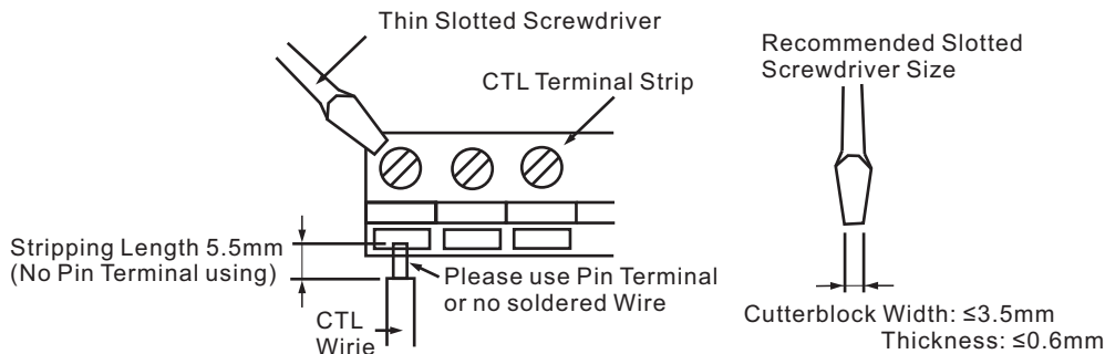
Fit CTL Wire into Terminal Strip
